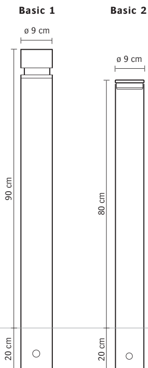
Potelet Basic 2
